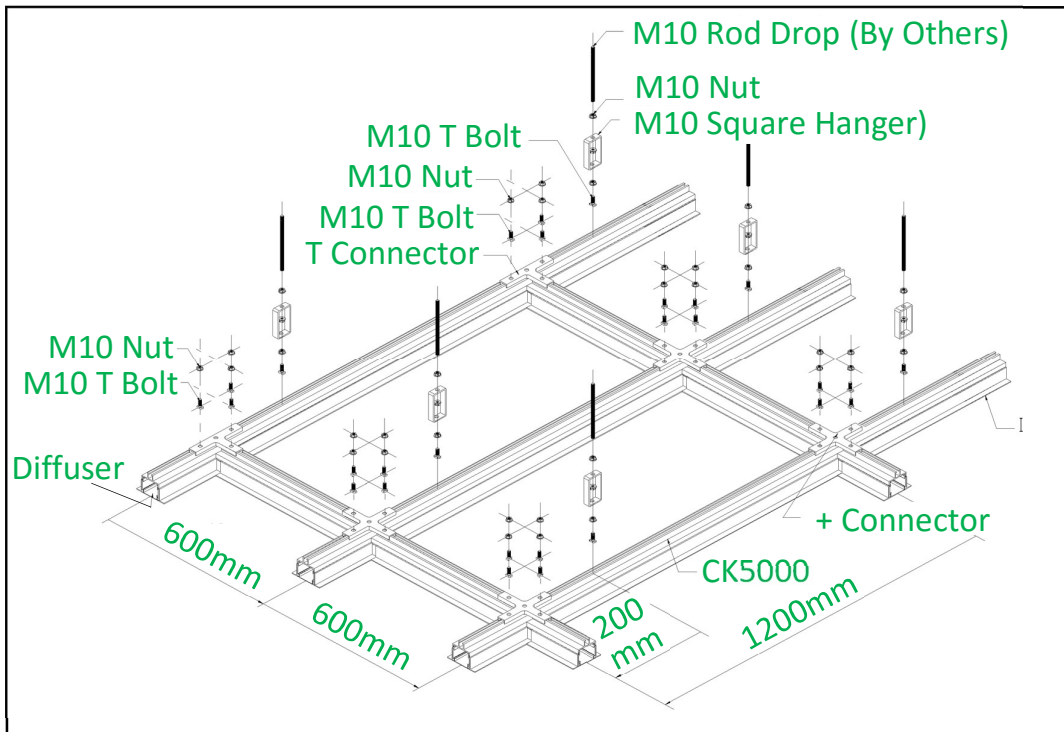
Figure 2: SK5000 Ceiling System Structure
