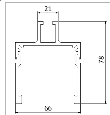
Figure 1: SK5000 Ceiling Grid
