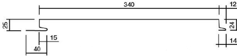
Figure 3: SP - GI DIVIDER APPEARANCE
