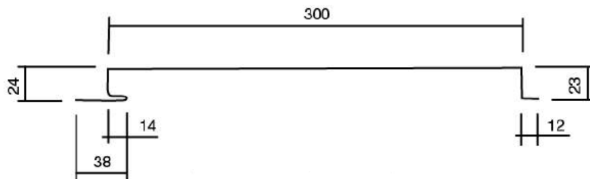
Figure 1: SP 300 - GI DIVIDER DIMENSION
